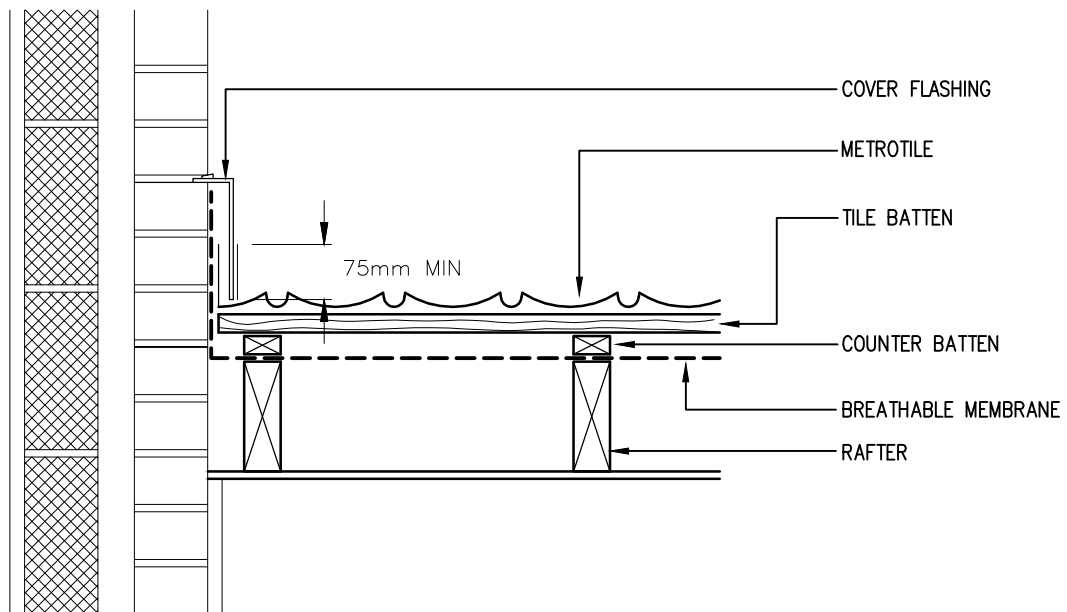
ALTERNATIVE DETAIL WITHOUT SIDEWALL FLASHING
