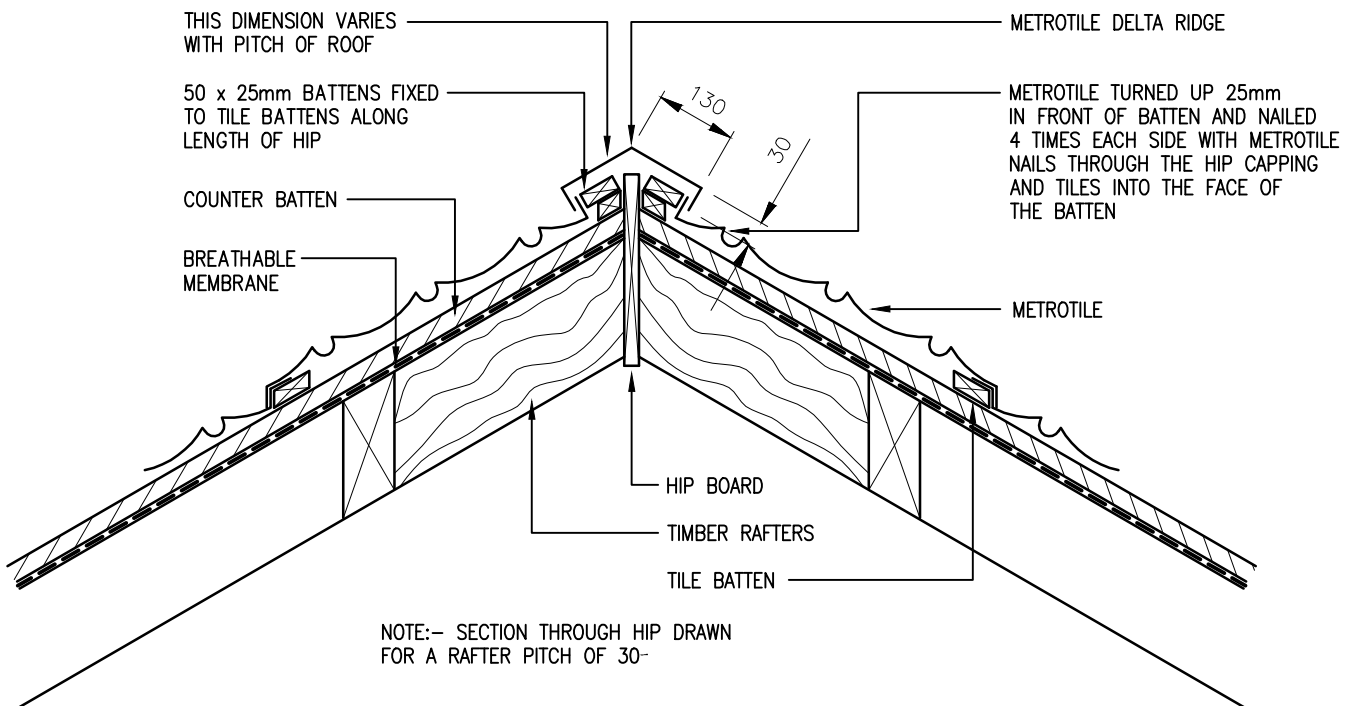
HIP DETAIL DELTA RIDGE/HIP
