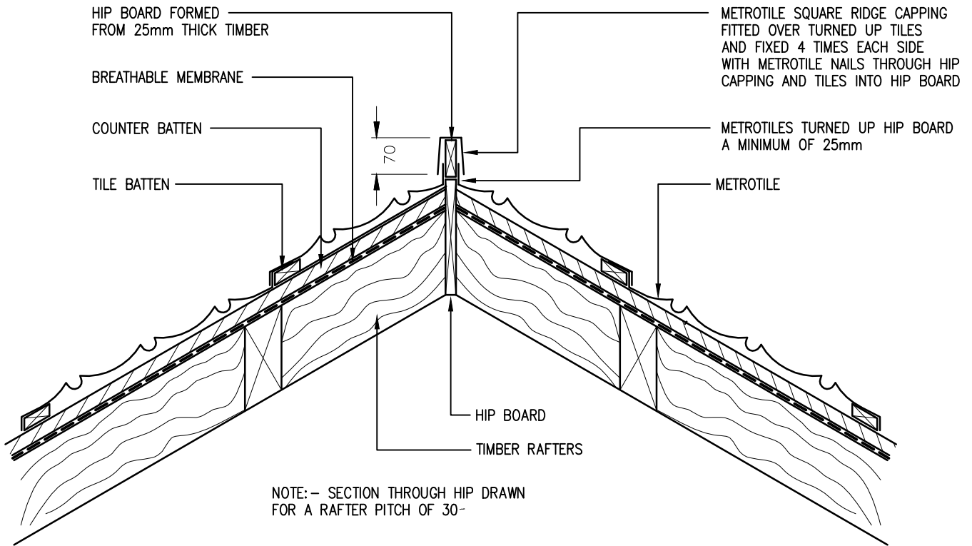
HIP DETAIL SQUARE RIDGE/HIP
