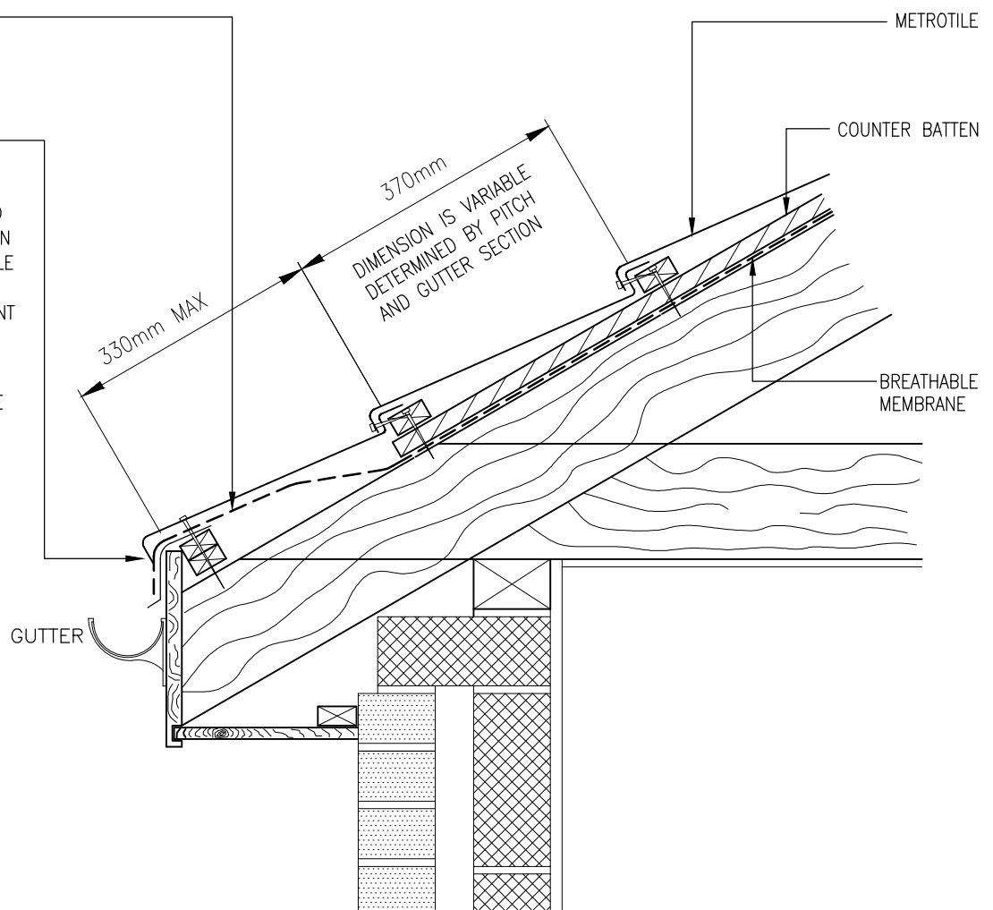
EAVES DETAIL
