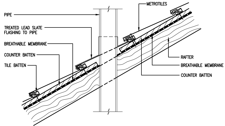
SOIL VENT PIPE THROUGH ROOF
