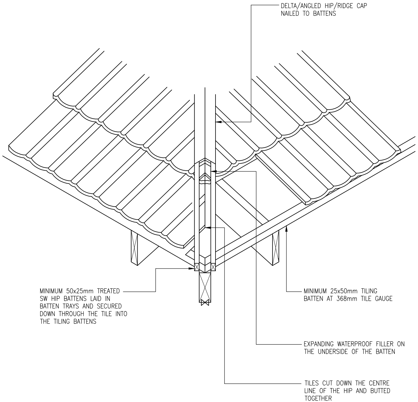
900 HIP DETAIL
