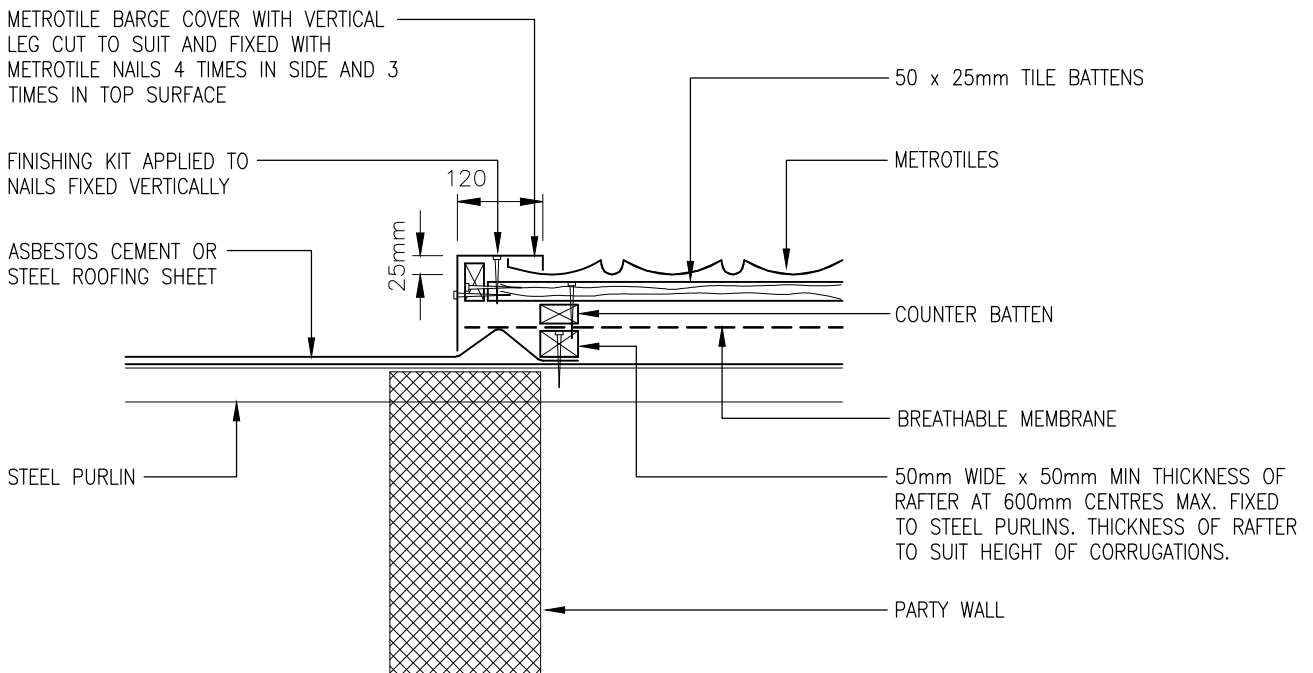
DETAIL OF METROTILE ABUTTING ASBESTOS OR STEEL SHEETING
