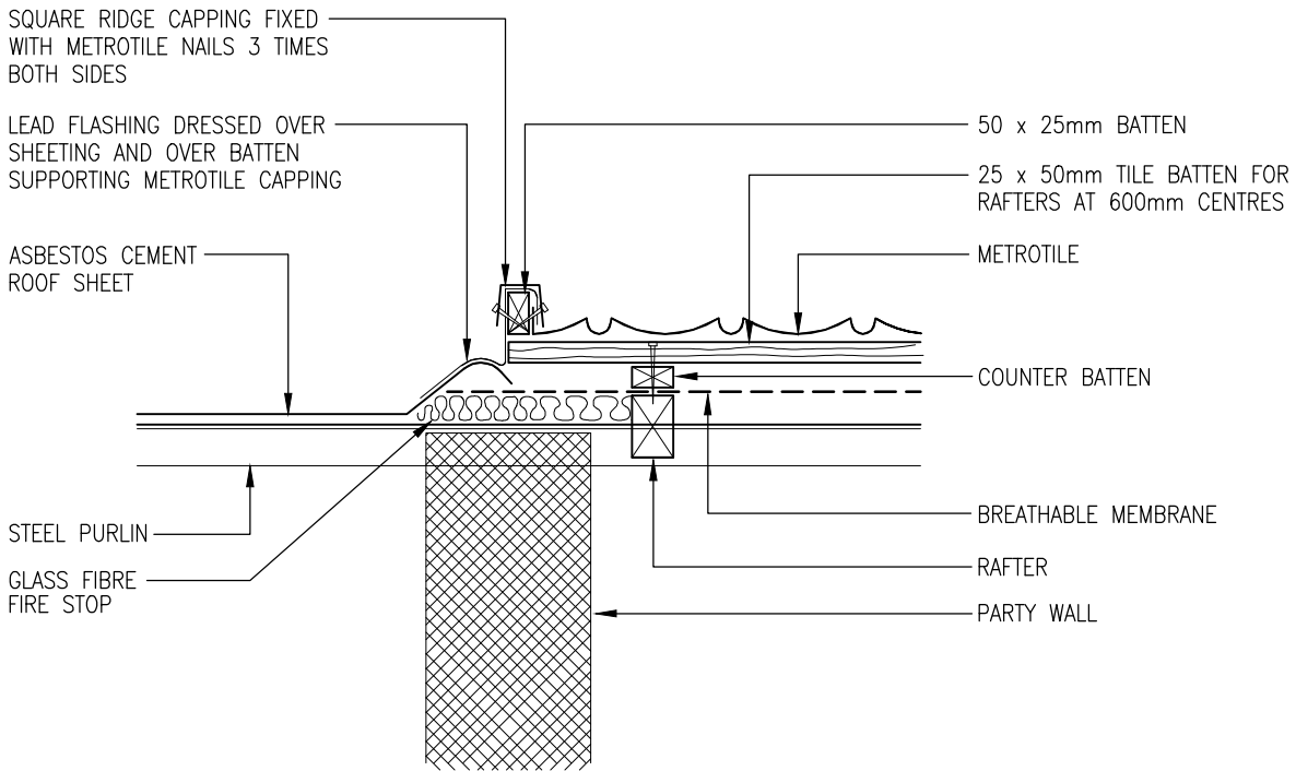
DETAIL OF METROTILE ABUTTING ASBESTOS SHEETS
