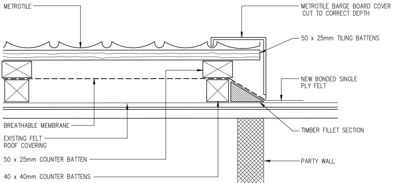
METROTILE JUNCTION WITH EXISTING FELT ROOF
