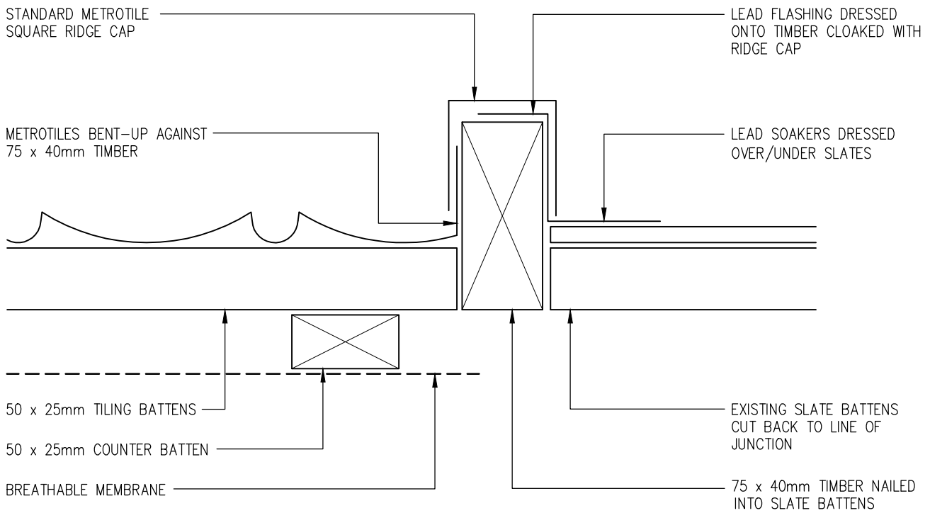
JUNCTION BETWEEN METROTILES & SLATE ROOFING
