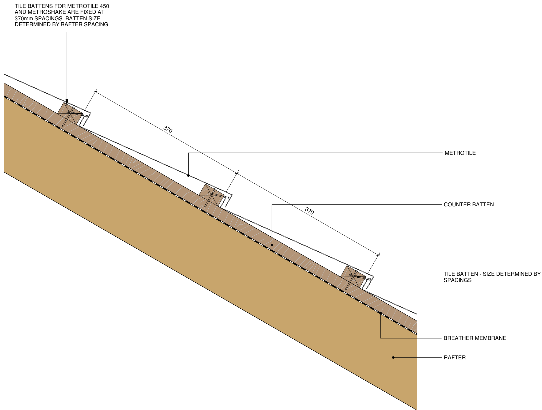
1 Metrotile Batten Spacing 1:5
