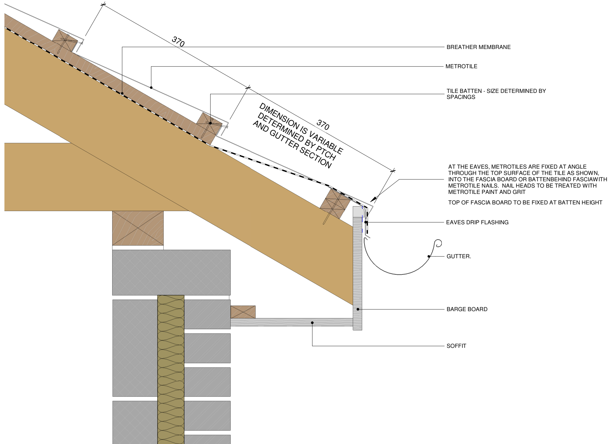
1 Metrotile Eaves Detail 1:5
