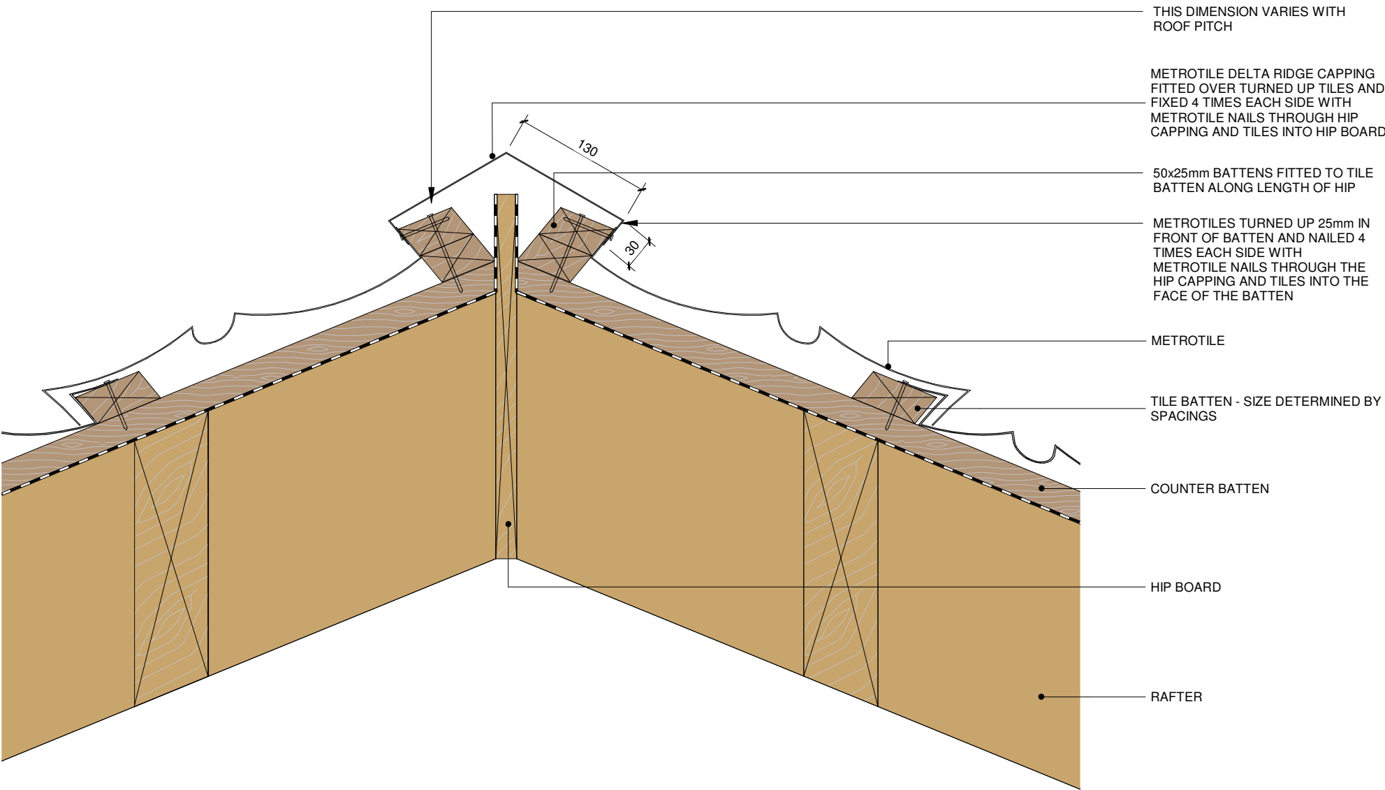
1 Metrotile Hip Delta Ridge Detail 1 : 5
