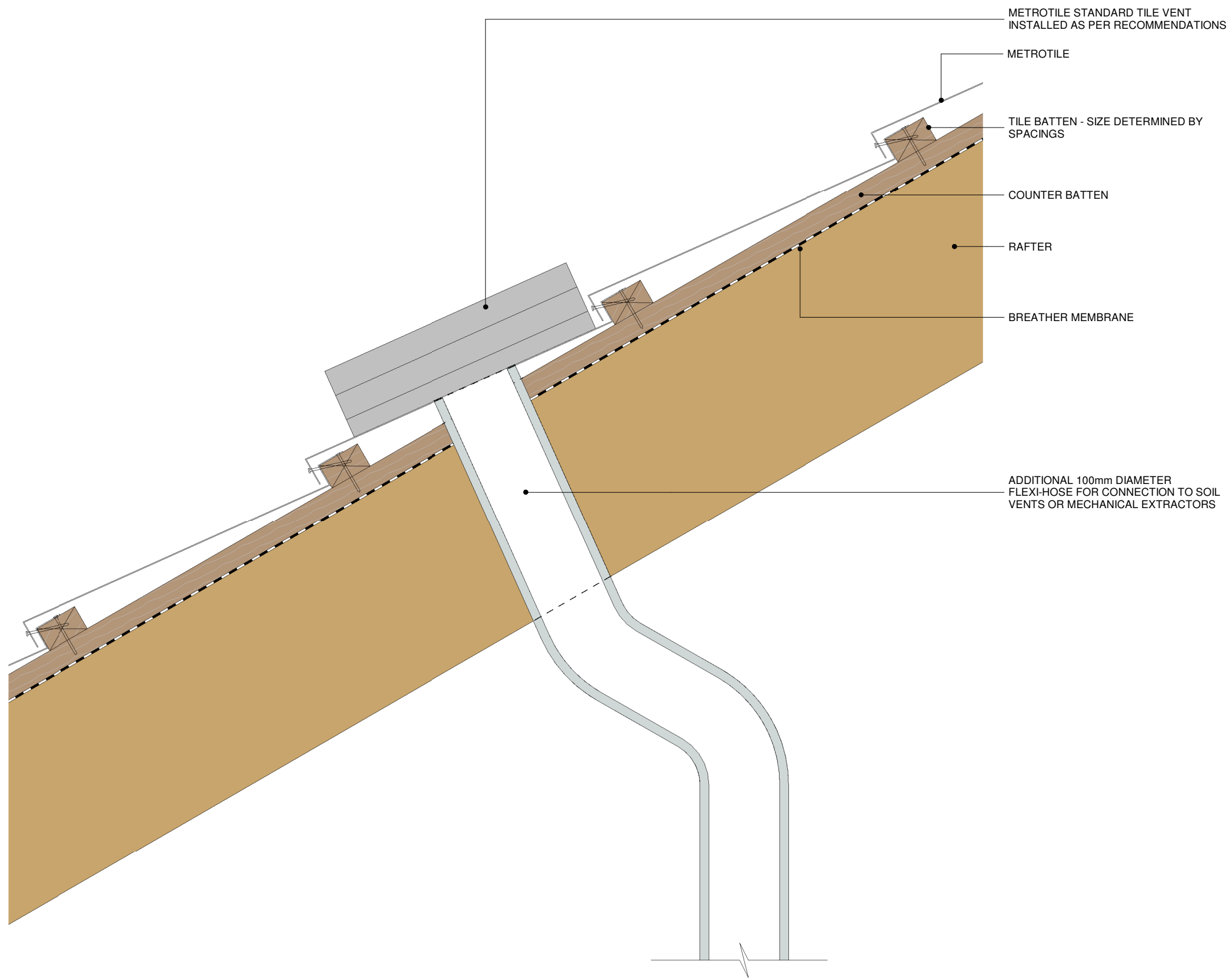
1 Tile Vent Pipe Detail 1:5
