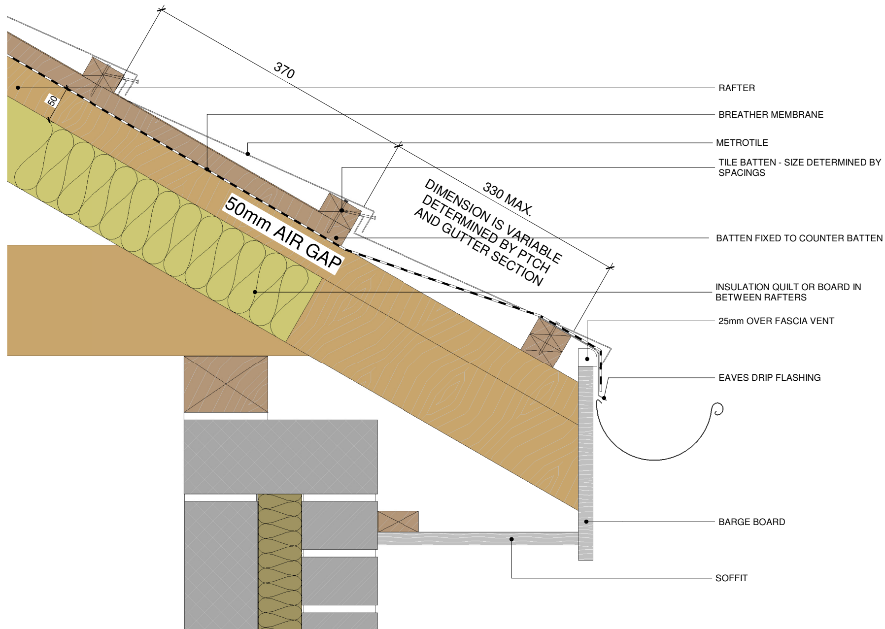
1 Metrotile Eaves Ventilation Detail 1:5
