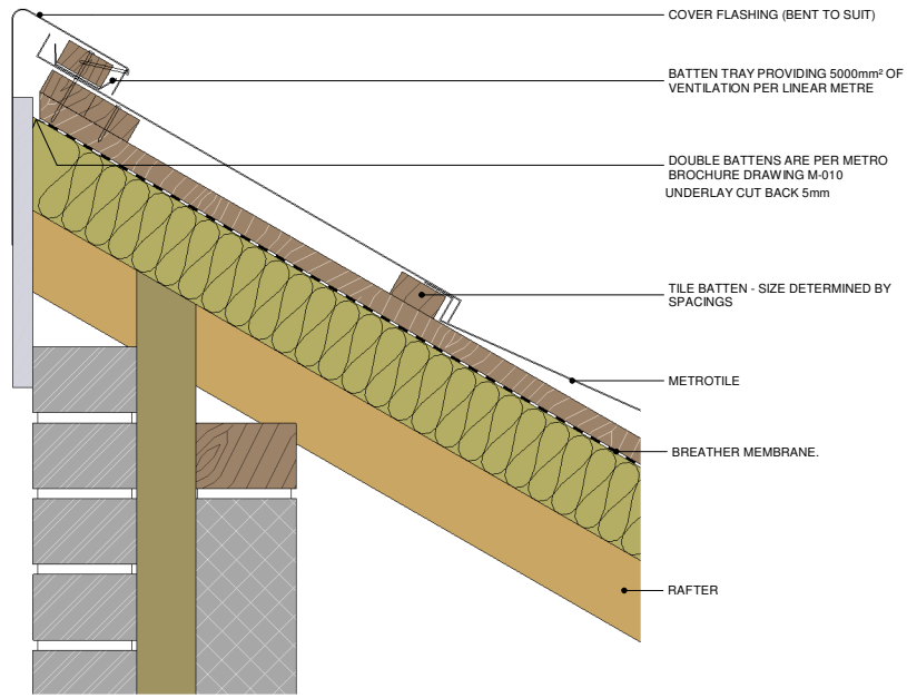
1 Metrotile Monoridge Detail 1:5
